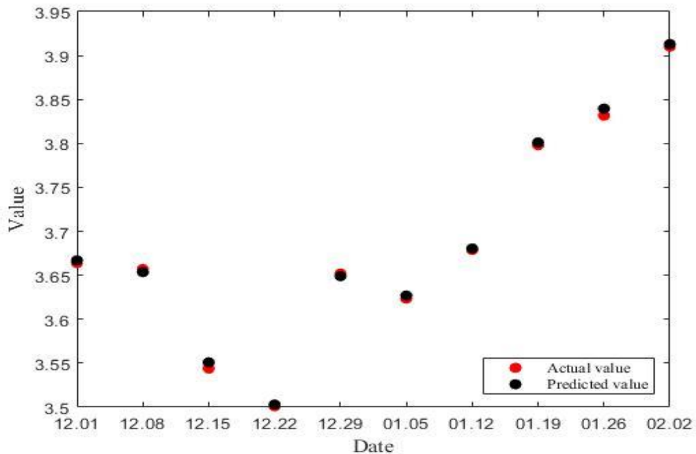
Figure 2. Weekly net fund neural network model prediction results
