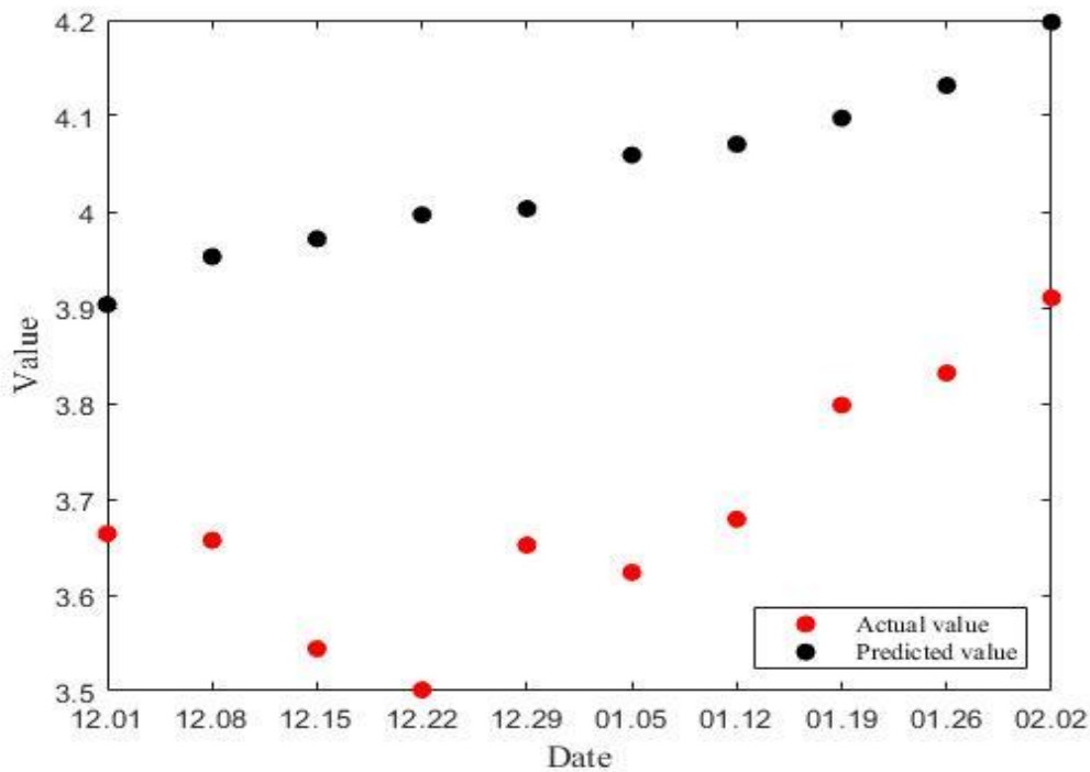
Figure 3. Grey model of fund net value predicts results
